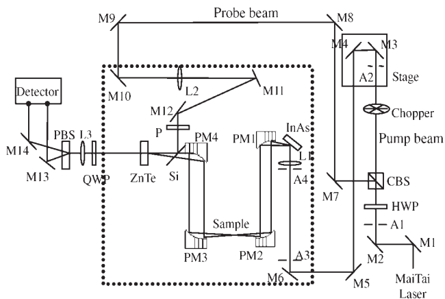
Figure 2: Diagram of the THz-TDS system
