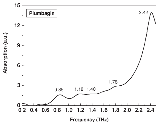
Figure 4: THz absorption spectra of plumbagin, juglone, and menadione.
