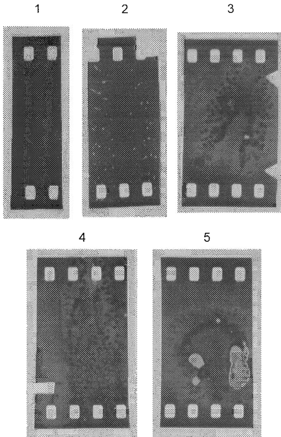
Figure 1: The film strips used to detect enzyme activity in various CP species.
